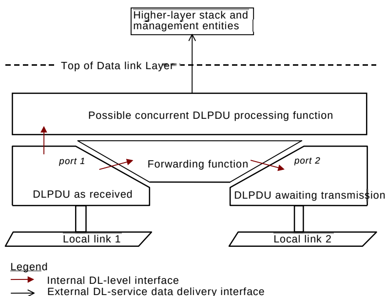
Figure 17 – Forwarding and delivering a received DLPDU
